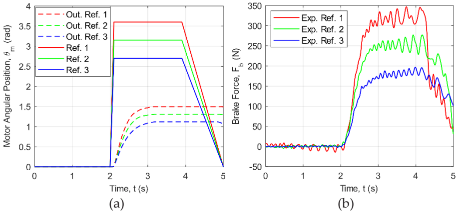
Figure 3: EWB prototype responses (a) Control target and actual (b) Brake force
