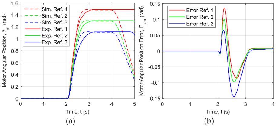
Figure 4: Motor angular position - simulation vs experimental (a) Response (b) Response error
