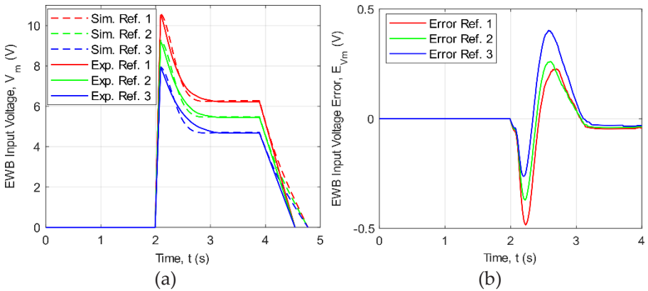
Figure 5: Motor voltage - simulation vs experimental (a) Response (b) Response error
