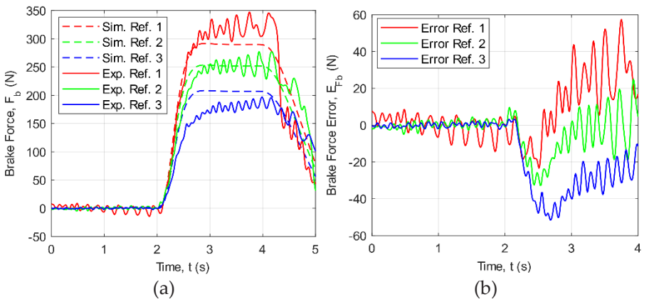
Figure 6: Brake force - simulation vs experimental (a) Response (b) Response error
