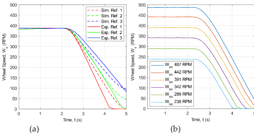
Figure 7: Wheel speed of test rig - simulation vs experimental (a) Different braking level (b) Different wheel speed
