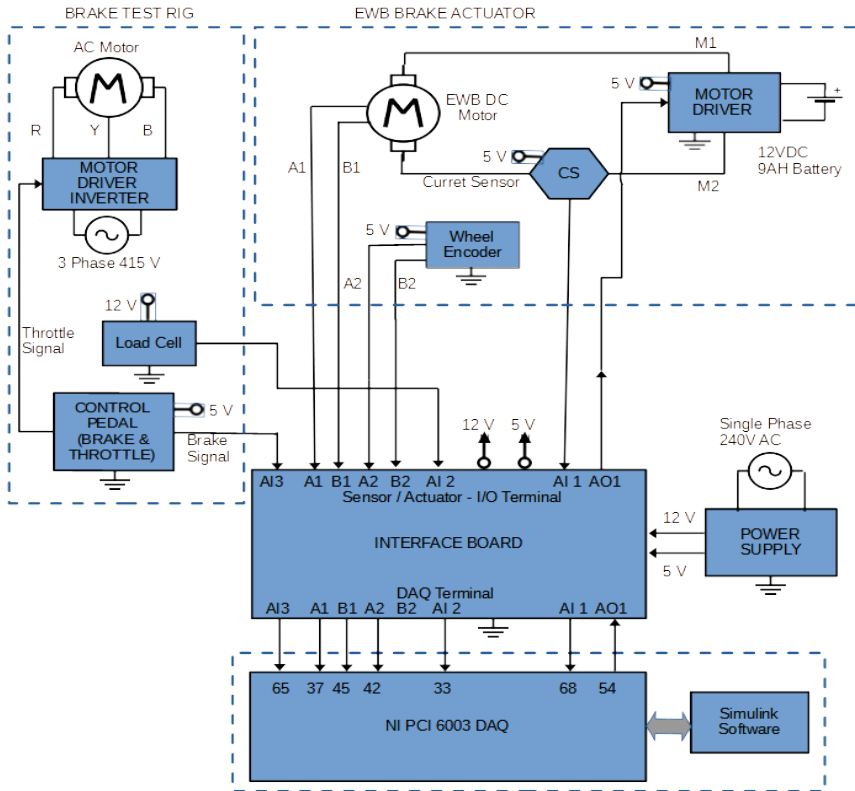
Figure 2: The EWB experimental wiring connection
