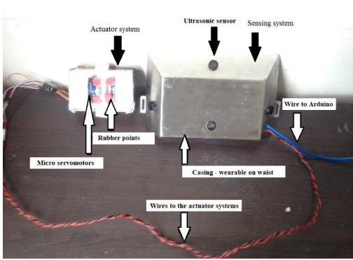
Fig. 11. Overall system
